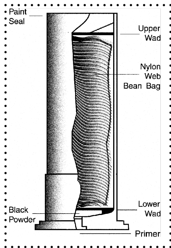
37mm bean bag round
