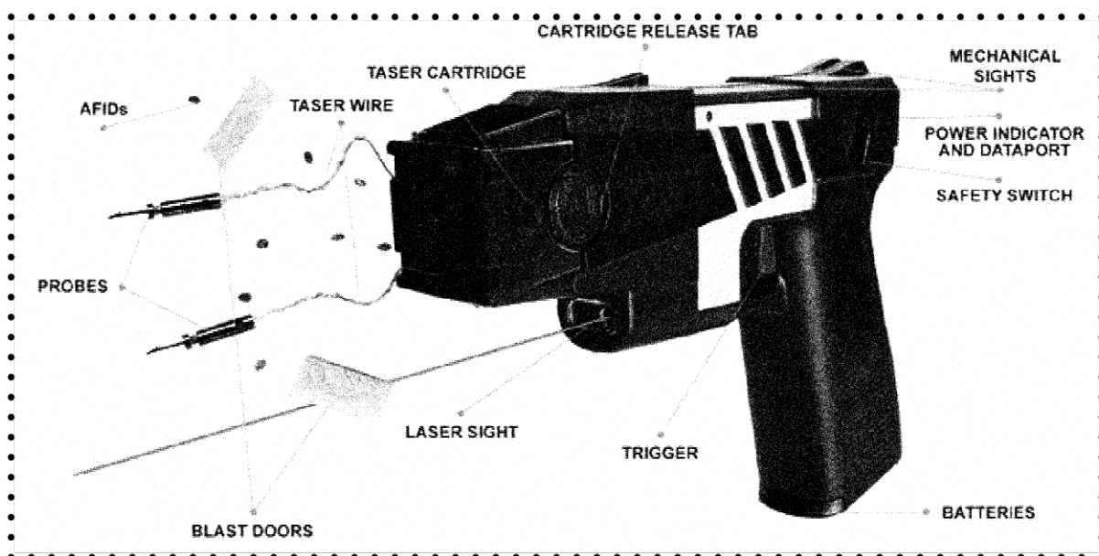
diagram of the TASER Advanced M26
