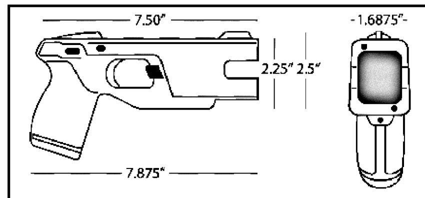
diagram of the TASER Advanced M26
