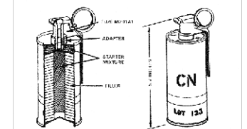
diagram of a tear gas canister
