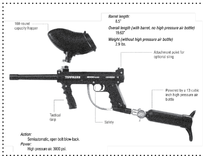
diagram of the PepperBall Custom Carbine Launcher
