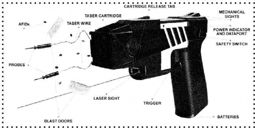
diagram of the TASER Advanced M26
