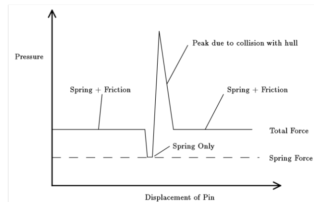
Figure 5.5: Pressure required to move pins
