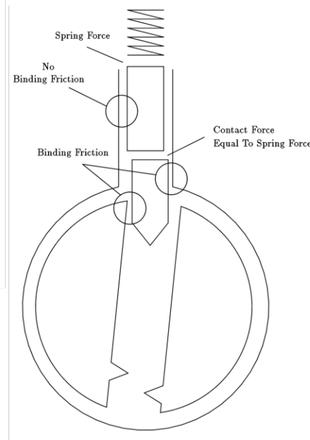
Figure 5.4: Key pin enters hull
