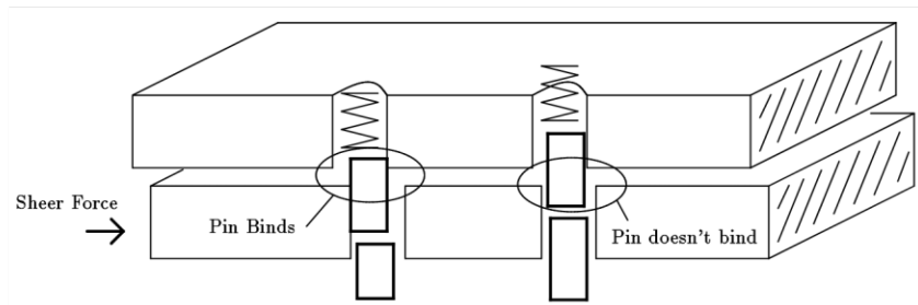
Figure 4.1: (a) Sheer force causes driver to bind
