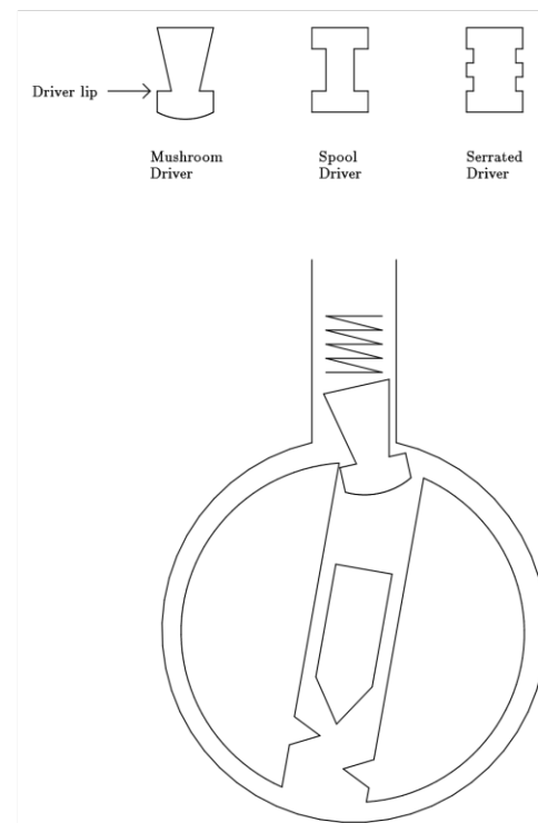
Figure 9.7: Mushroom, spool, and serrated driver pins
