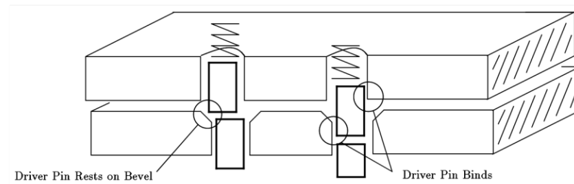
Figure 9.5: (a) Driver sets on bevel
