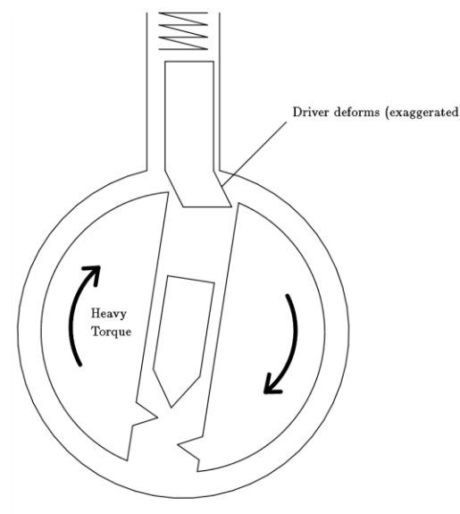
Figure 9.2: Driver pin false set by elastic deformation
