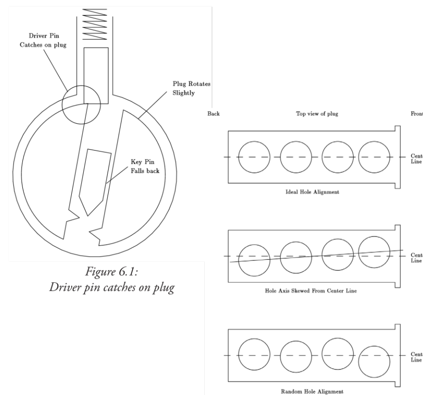
Figure 6.2: Alignment of plug holes
