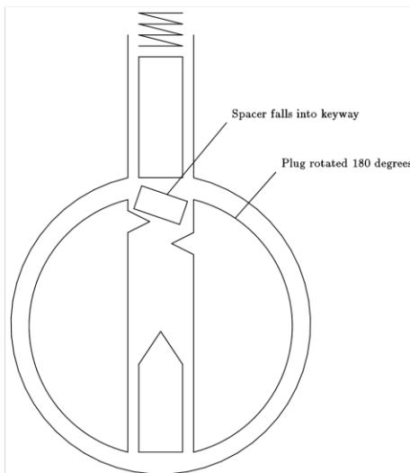
Figure 9.9: Spacer or driver can enter keyway
