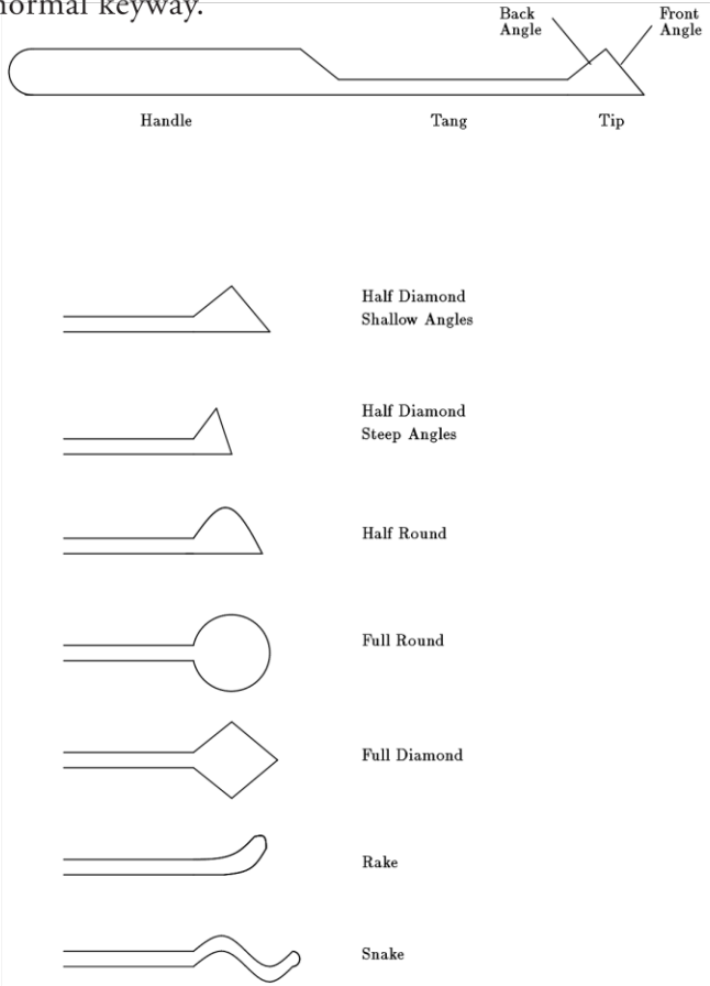
Figure A.1: Selection of pick shapes
