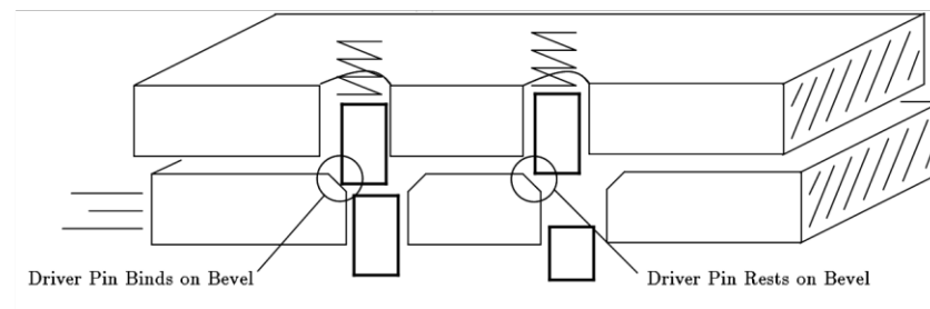
Figure 9.6: (b) Driver jams on bevel
