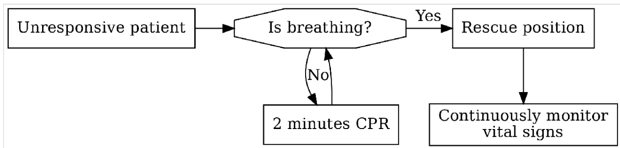
Figure 3: BLS Flowchart
